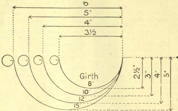
Sections showing dimensions of each size.
